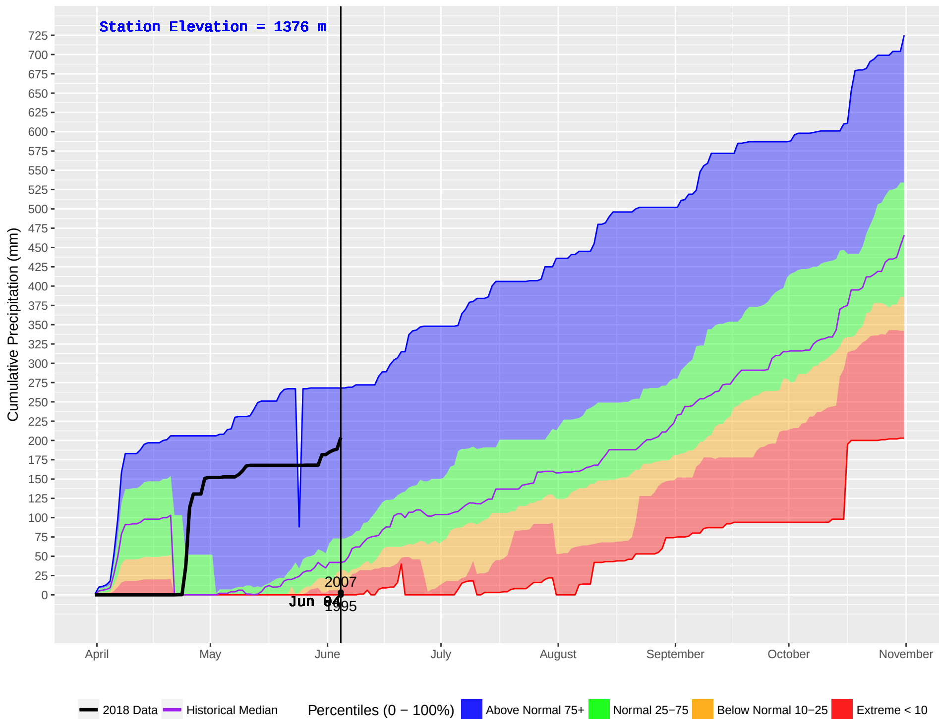
DUNCAN (385) : Historical (1981–2016) and Current (2018) Noon Cumulative Precipitation
