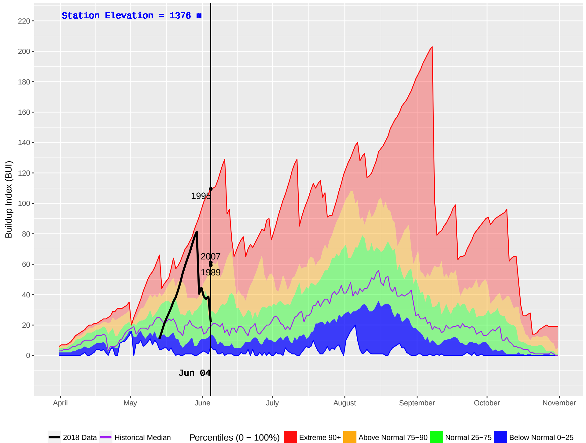
DUNCAN (385) : Historical (1981–2016) and Current (2018) Noon Buildup Index (BUI)
