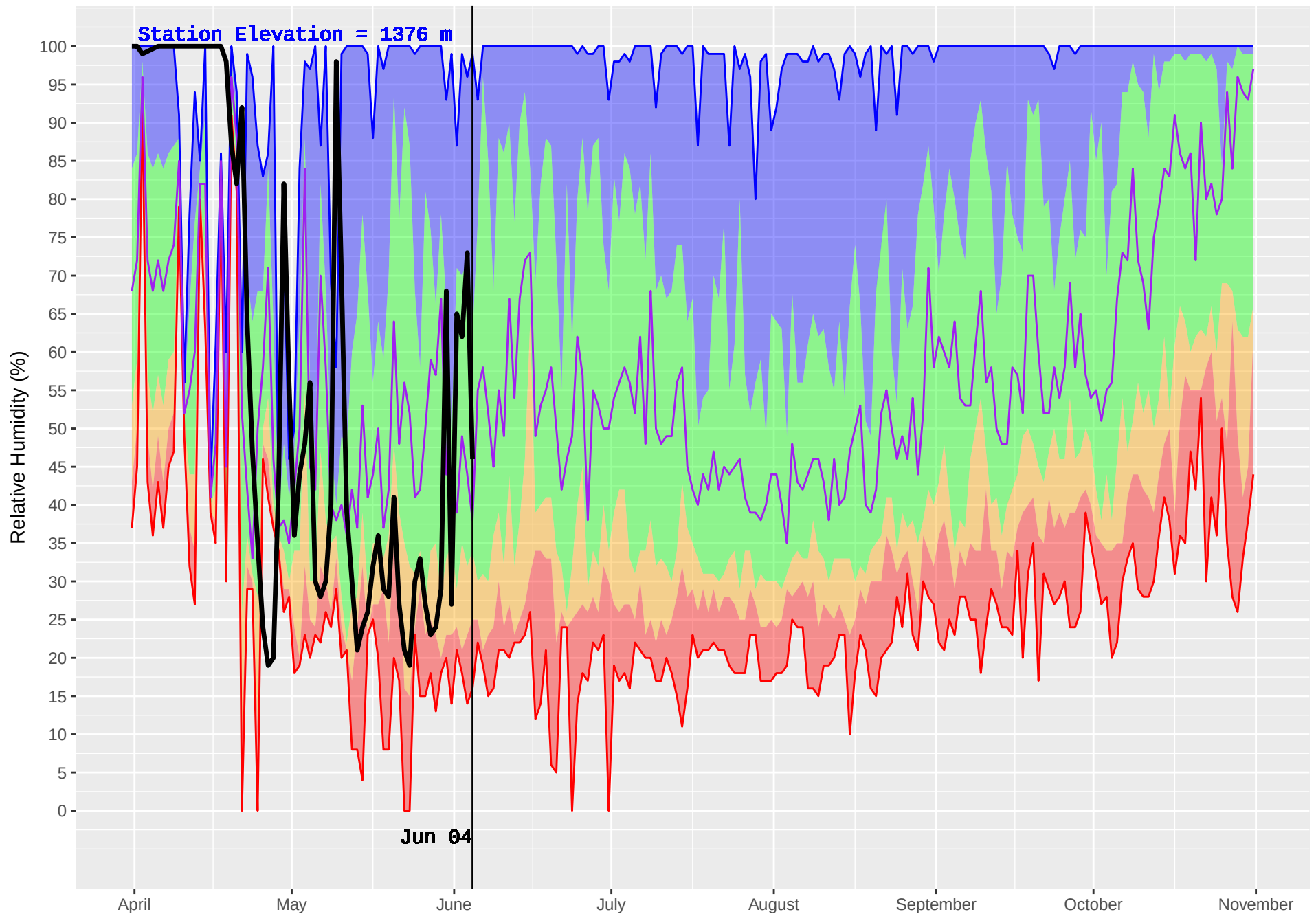
DUNCAN (385) : Historical (1981–2016) and Current (2018) Noon Relative Humidity
